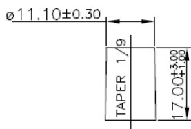
NEGATIVE TERMINAL
